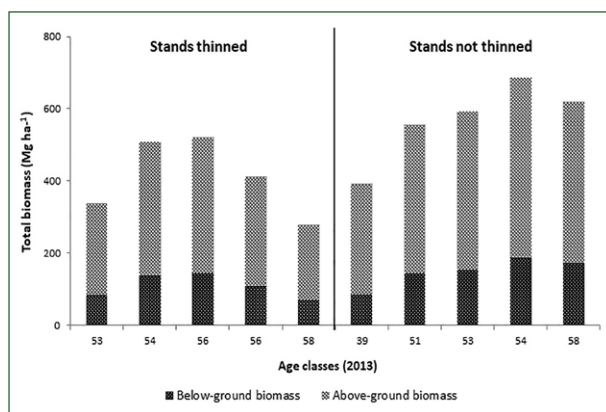
Figure 5 - Total biomass distribution relating to the different ages of the Calabrian pine stands in 2013.
