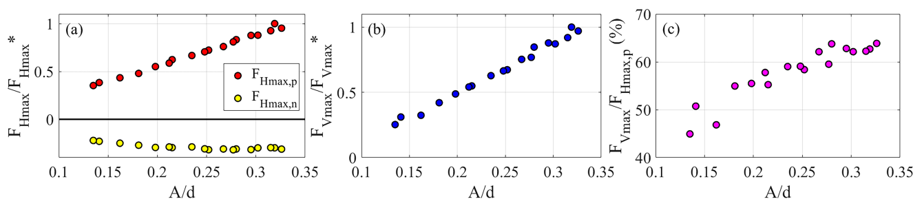
Figure 7. Maximum positive and negative wave forces vs. A/d . (a) Horizontal force; (b) vertical force; (c) weight of the vertical force with respect to the horizontal one.
