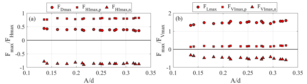
Figure 13. (a) Maximum Morison force components vs. A/d : positive drag F_{Dmax} , positive horizontal inertia F_{HImax,p} and negative horizontal inertia F_{HImax,n} ; (b) maximum transverse force components vs. A/d : positive lift F_{Lmax} , positive vertical inertia F_{VImax,p} and negative vertical inertia F_{VImax,n} .
