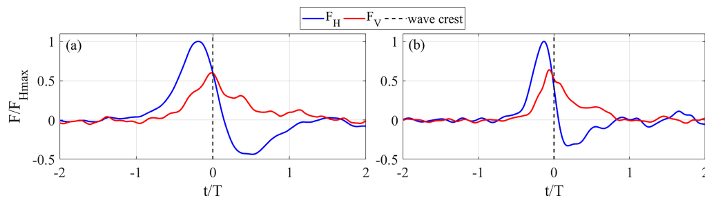
Figure 6. Time variation of horizontal F_H and vertical F_V wave forces vs. A/d . (a) Test no. 8; (b) test no. 18.
