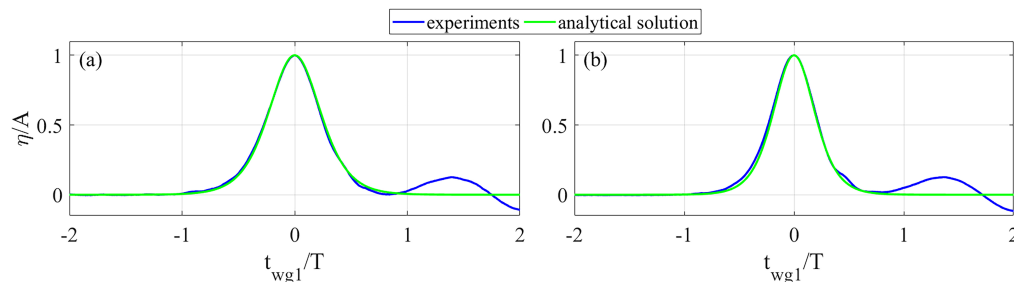
Figure 3. Comparison between experimental and analytical time series of surface elevation \eta at wg1. (a) Test no. 8; (b) test no. 18.
