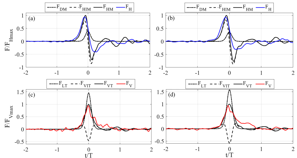
Figure 12. Experimental and calculated time series of hydrodynamic forces. (a) Comparison between experimental F_H and Morison F_{DM} , F_{HIM} and F_{HM} (test no. 8); (b) comparison between experimental F_H and Morison F_{DM} , F_{HIM} and F_{HM} (test no. 18); (c) comparison between experimental F_V and transverse F_{LT} , F_{VIT} and F_{VT} (test no. 8); (d) comparison between experimental F_V and transverse F_{LT} , F_{VIT} and F_{VT} (test no. 18).
