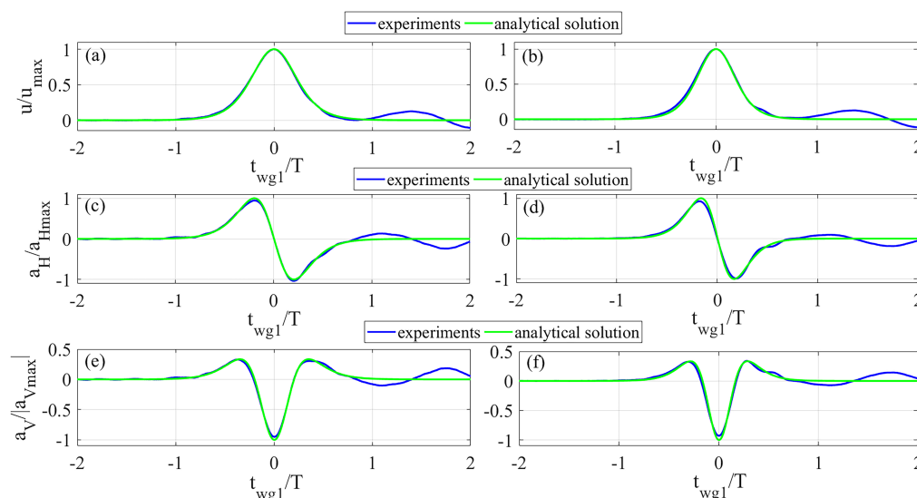
Figure 4. Comparison between experimental and analytical time series of kinematic field at wg1. (a) u (test no. 8); (b) u (test no. 18); (c) a_H (test no. 8); (d) a_H (test no. 18); (e) a_V (test no. 8); (f) a_V (test no. 18).
