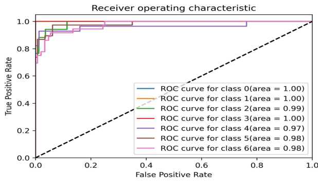
FIGURE 8. ROC curve obtained on SAVEE dataset using our proposed model.
