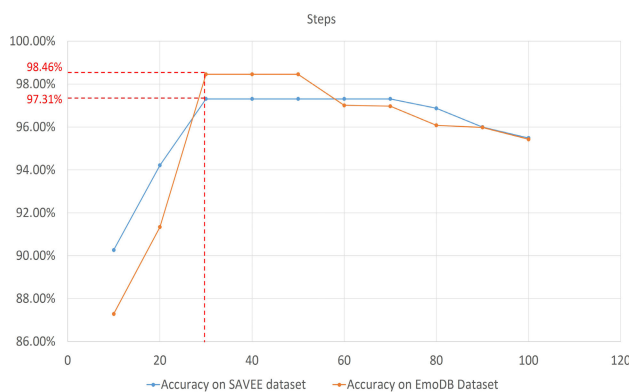
FIGURE 14. Variation of accuracy on SAVEE and EmoDB datasets with respect to steps or the number of iterations for XGBoost classifier.
