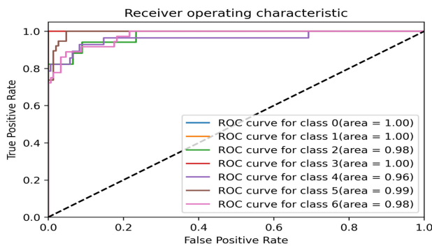
FIGURE 9. ROC curve obtained on EmoDB dataset using our proposed model.
