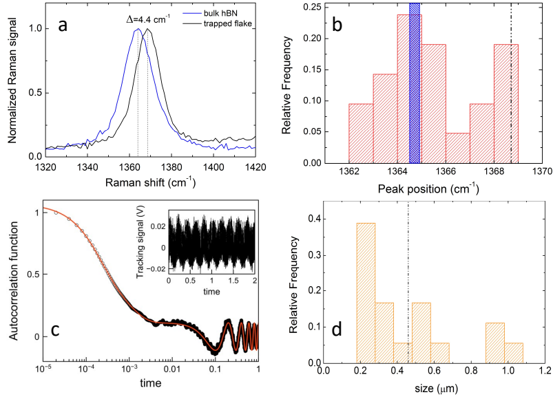
Figure 2: Spectroscopy, trapping and metrology of hBN flakes. (a) Comparison between the Raman spectra of bulk hBN (blue curve) and trapped hBN monolayer (black curve). The blue shift \Delta of the Raman peak of the monolayer with respect to the bulk value is also indicated. The exciting wavelength was \lambda=780 nm. (b) Histogram of the Raman peak position of the trapped hBN flakes. The Raman peak positions \Delta_0 = 1364.7 \text{cm}^{-1} and \Delta_0 = 1368.6 \text{cm}^{-1} due to the bulk and the monolayer, respectively, are also indicated (blue bar and black dashed line). (c) Transverse signal autocorrelation function (black points) and its fit (red curve) with a double exponential decay plus a sinusoidal oscillation at \omega_{stage} . (d) Distribution of hBN flake size. The mean flake diameter d (dash-dot line) is approximately 460 nm. Bin size 100 nm, smallest diameter 180 nm.
