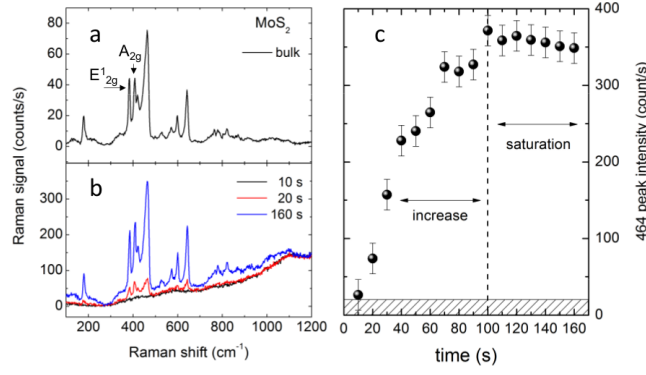
Figure 4: Optical force aggregation of MoS 2 . Raman spectra obtained on bulk MoS 2 (a) and under laser pushing of exfoliated MoS 2 at 638 nm (b). In (a), a long-working distance (LWD) \times 50 objective (NA=0.5) has been used, while in (b) a \times 100 oil immersion objective (NA=1.3) has been used. (c) Time evolution of 2LA(M) peak at \Delta_0 \approx 464 \text{ cm}^{-1} shown in (b). A clear increase of the peak signal is observed in the first 100 s of the pushing process, followed by its stabilization and saturation, due to the complete filling of the sampling volume of laser beam.
