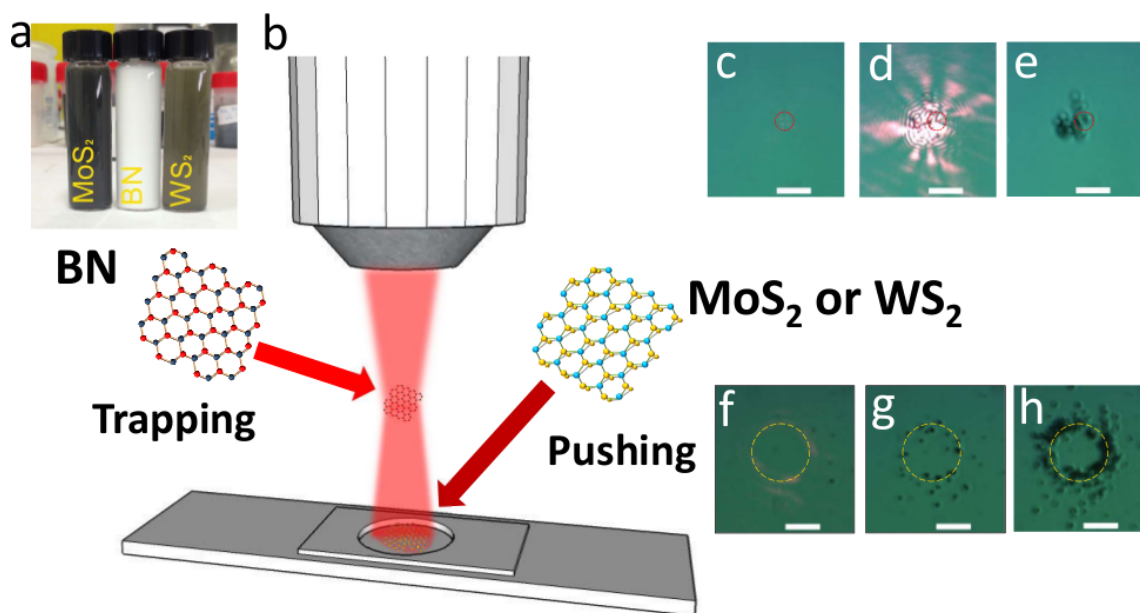
Figure 1: (a) Aqueous dispersions of the 2D materials. (b) Sketch of the experimental setup. A high numerical aperture objective (NA = 1.3) is used to obtain a diffraction limited spot. Particles are trapped in the laser focus when the optical gradient force is greater than the scattering force. Conversely, the particles are optically pushed toward the bottom of the sample cell. If BSA is diluted in the aqueous medium, the particles stick to the walls of the cell and surface patterning is obtained. (c)-(e) Optical microscope images recorded at the beginning of the pushing process of WS 2 with a Gaussian beam (c) and after approximately 90 seconds (d, e). In (d), the scattering of the laser light due to the formation of the WS 2 aggregate is clearly observed. The dashed circles are guides for the eye indicating the location of the beam waist. (f)-(h) Optical microscope images registered at the beginning of the pushing process of MoS 2 (f) with a Laguerre-Gauss beam ( l = 30 ), after approximately 2 minutes (g) and after approximately 18 minutes (h). The dashed circles are guides for the eye indicating the location of the high intensity doughnut beam (see also Supplementary Video 3).
