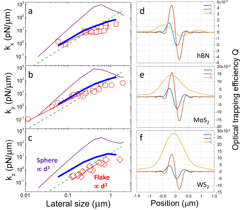
Figure 3: (a-c) Optical trap force constants k_x (red squares), k_y (red circles) and k_z (red diamonds) measured for trapped hBN flakes as a function of their lateral size determined from the autocorrelation analysis (note the log-log scale). Optical force measurements are obtained at 830 nm with 26 mW power at the sample. Red lines are a power law fit to the small size data consistent a size scaling of d^2 . Purple lines are Mie theory calculations for a sphere, following a d^3 scaling for small size. The dashed green lines represent the force constant estimates based on a simple dipole approximation (see ESI). Blue thick lines are T-matrix calculations for a planar cluster model of the hBN flake oriented in the xz plane because of optical torque. The agreement between experiments and T-matrix theory is excellent with no free parameters. (d-f) T-matrix calculations (830 nm, NA=1.3) of optical force efficiencies, Q_x (light blue), Q_y (red), and Q_z (yellow) for 0.9 \mu\text{m} planar clusters of hBN (d), MoS 2 (e), and WS 2 (f). Note how Q_z has no zero for the case of MoS 2 and WS 2 , hence trapping is not possible because of the strong absorption of these materials in the near-infrared.
