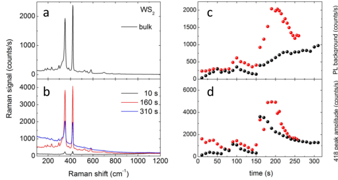
Figure 5: Optical force aggregation of WS 2 . On the left, Raman spectra obtained on bulk WS 2 (a) and under laser pushing of exfoliated WS 2 (b). For the spectrum of the bulk, the \times 50 LWD objective has been used. On the right, the time evolution of the photoluminescence background (c) and of the \Delta_0 \approx 417 \text{ cm}^{-1} Raman peak (d) of WS 2 for two different pushing powers (black dots, \sim 5 \text{ mW} ; red dots, \sim 17 \text{ mW} ) are shown. In these plots, the error bars are smaller than the data marker size. Exciting wavelength \lambda = 638 \text{ nm} .
