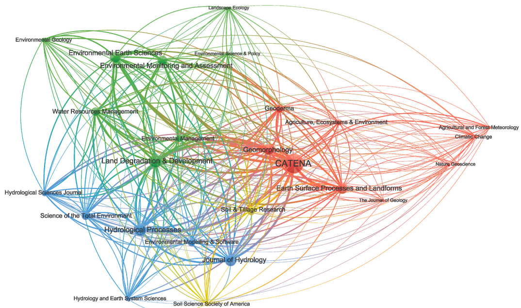
Fig. 7. Bibliographic coupling of journals with more than 250 citations where the network shows the relatedness of journals based on the number of shared references. The size of the circle indicates a weight of the item, the lines indicate the links among items, the distance among items shows their relatedness and different colours indicate clusters. (For interpretation of the references to colour in this figure legend, the reader is referred to the Web version of this article.)
