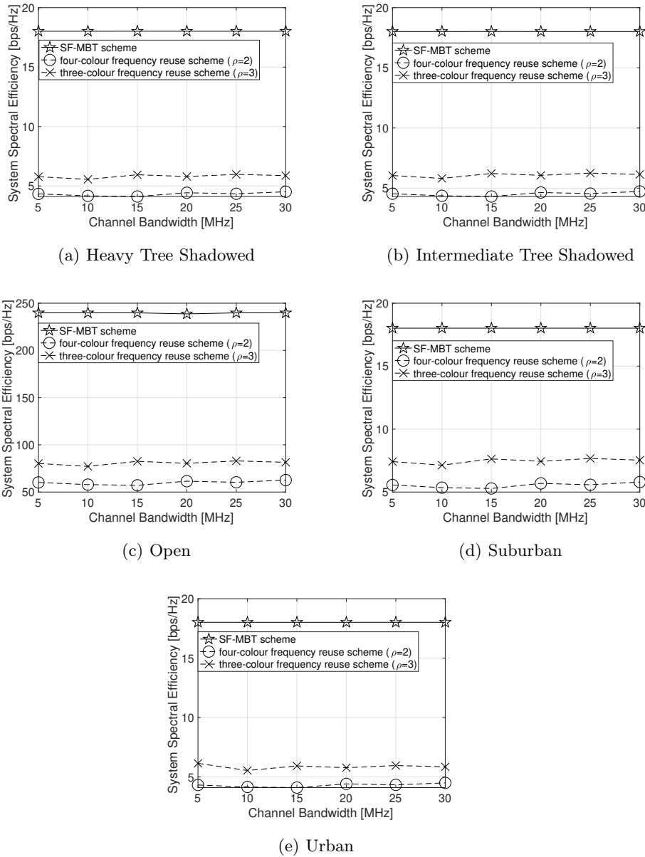
Fig. 4.8. System spectral efficiency for SF-MBT, four-color, and three-color frequency re-use schemes with a varying channel bandwidth.
