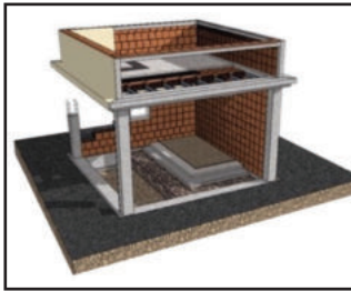
Figure 2 - Prototype Building. Common Scenario. Source: Authors.
