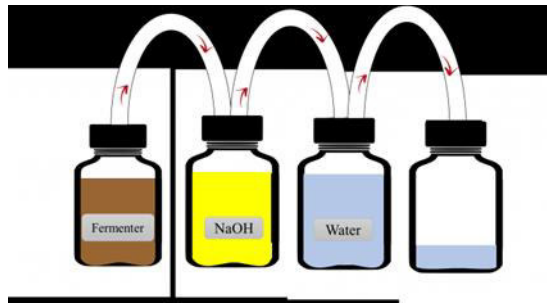
Figure 5.1 Graphical set-up of the BMP test with water displacement method for biomethane quantitation.
