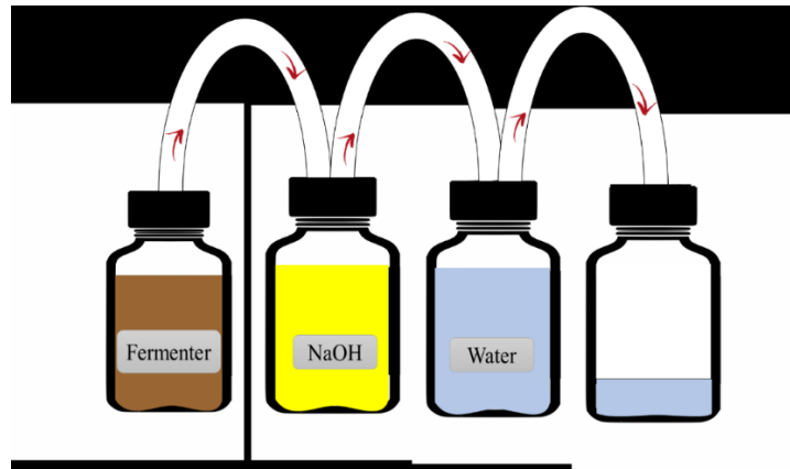
Figure 3.11 Setting up the reactors
