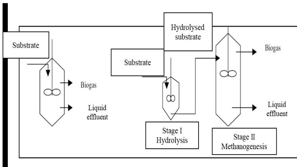
Figure 2.1 One-stage and two-stage AD process.
