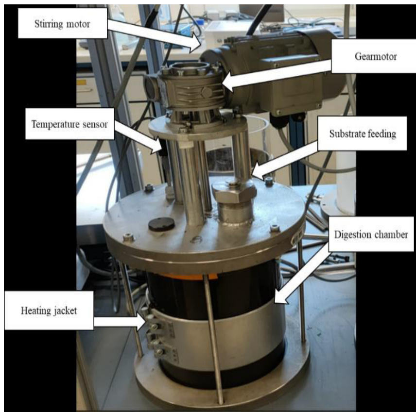
Figure 3.13 Reactor set-up
