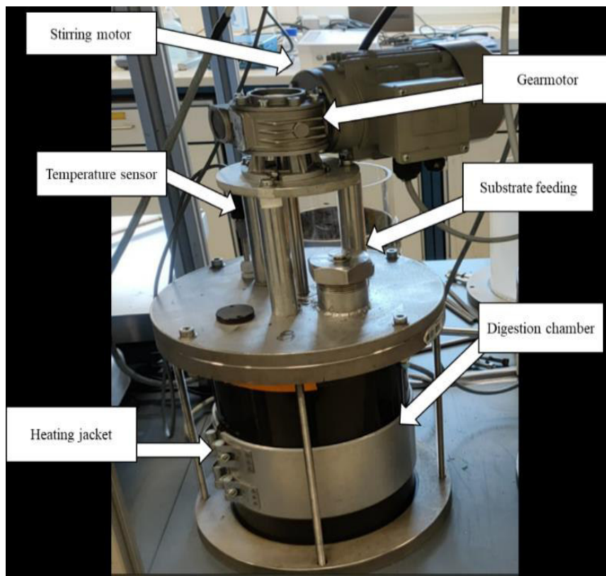
Figure 7.1 Reactor set-up
