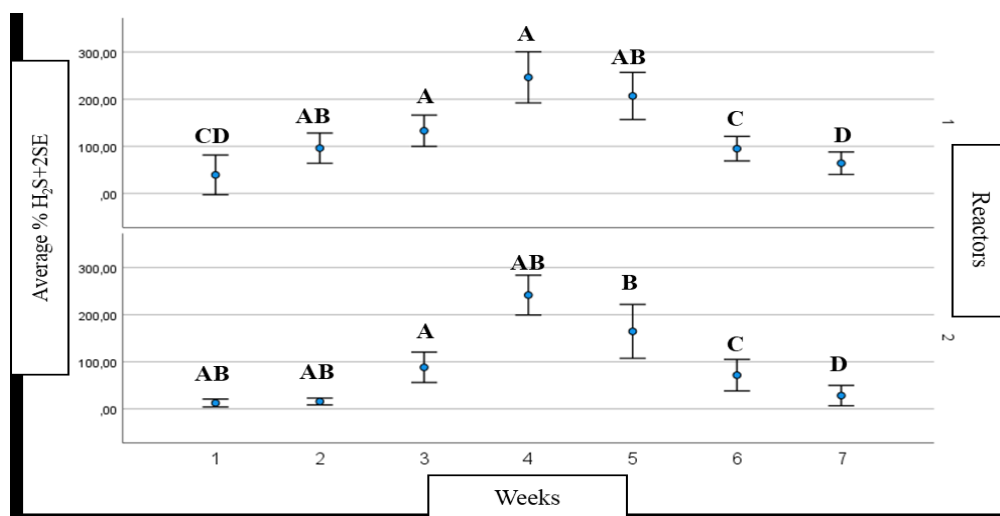
Figure 7.12 Variation in percentage concentration of H 2 S during the trial weeks. Data marked with different capital letters are significantly different by Tukey's test ( p < 0.05 )
