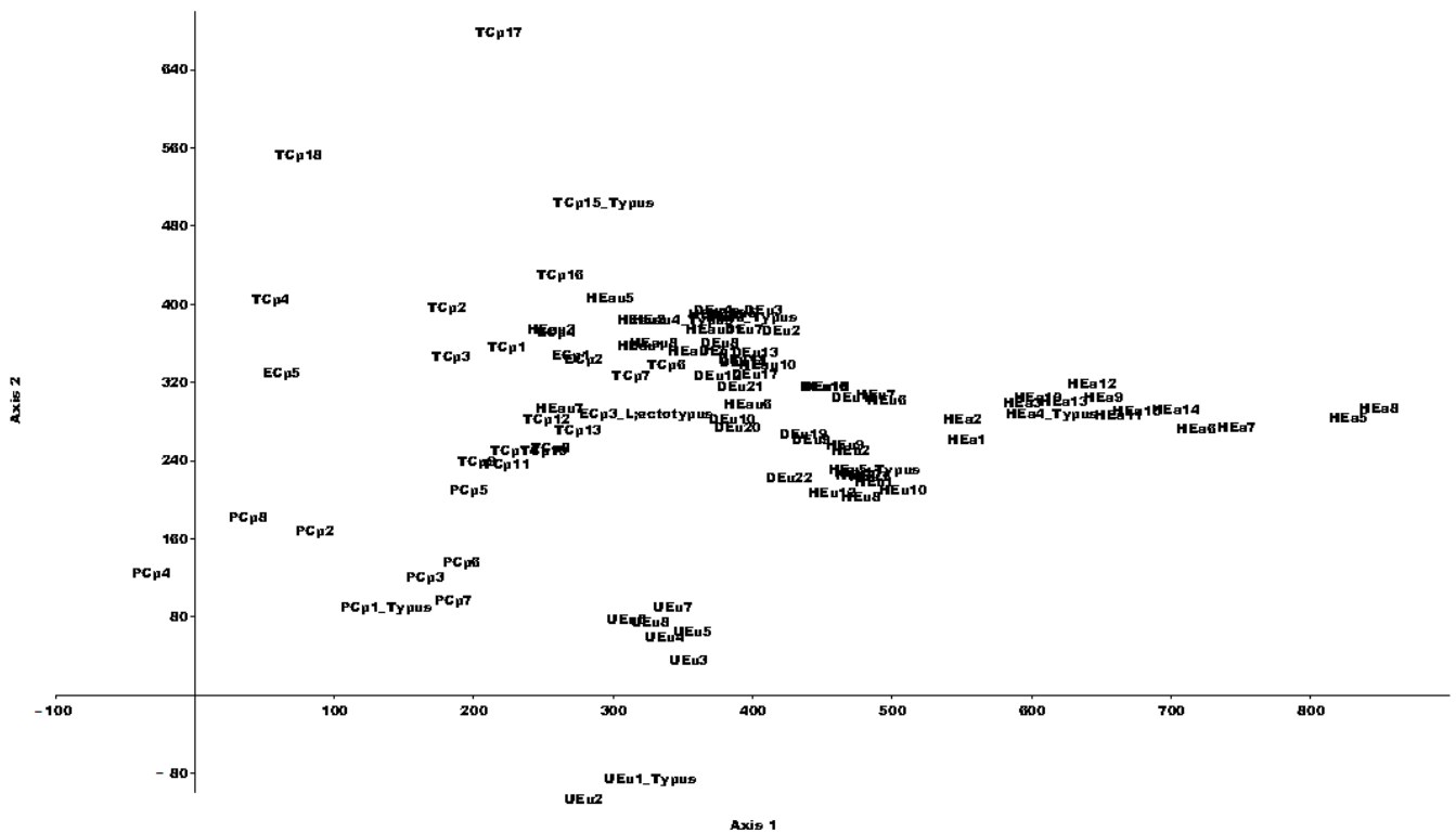
Figure 5. DCA ordination of heathland communities in the central-western Iberian Peninsula.
