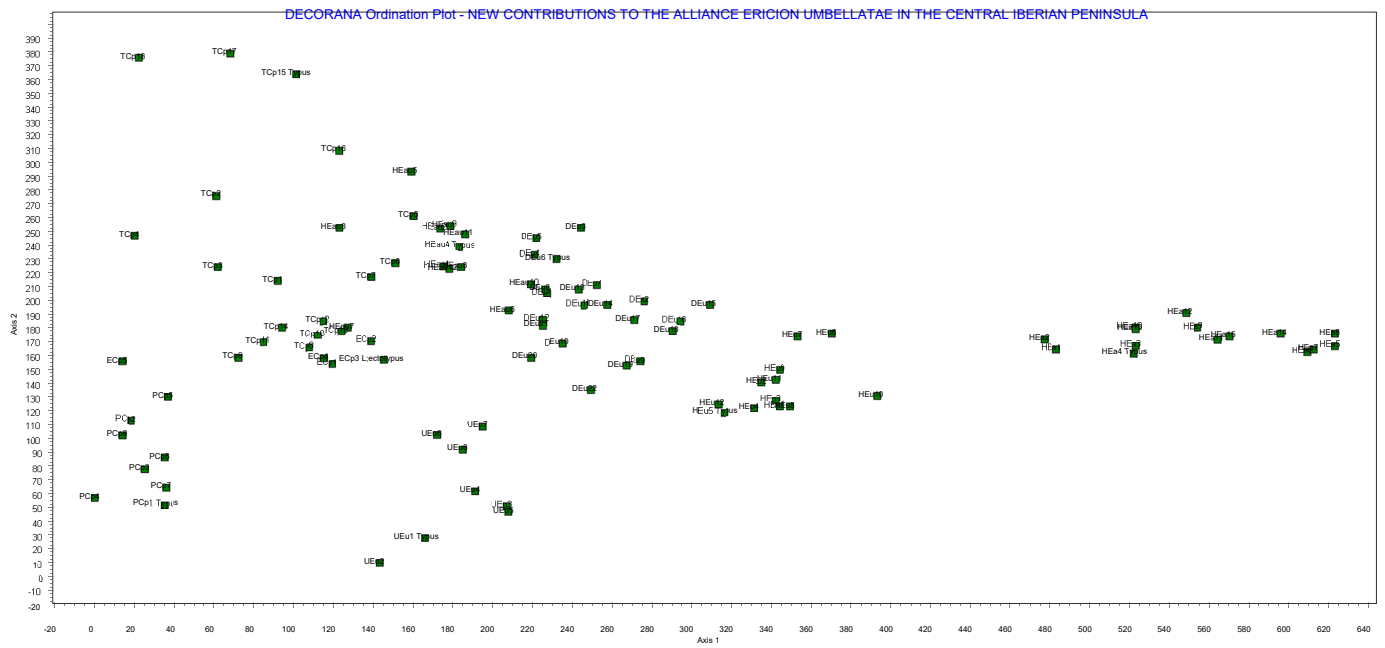
Figure 4. DECORANA (Detrended analyse of variance) ordination of heathland communities in the central-western Iberian Peninsula.
